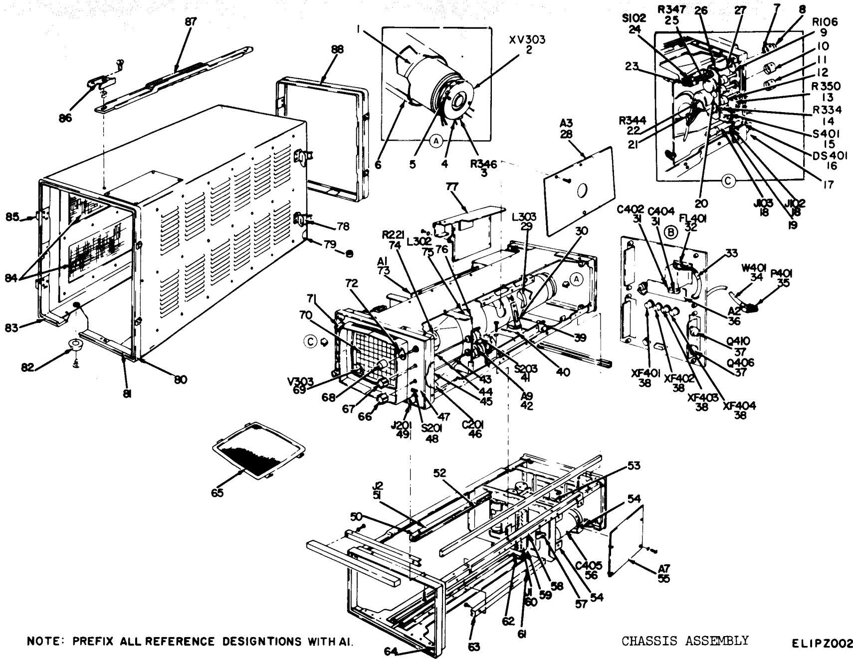
Figure 2. Oscilloscope Assembly OS-189A(P)/USM-281 (Sheet 1 of 2).
