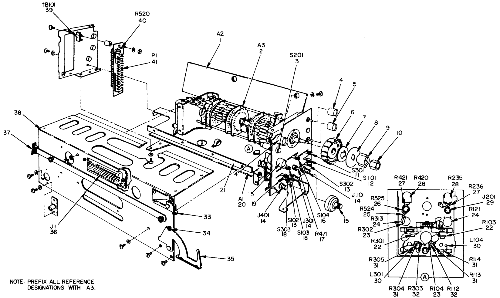
Figure 18. Plug-In Unit, Time and Base Oscilloscope.
