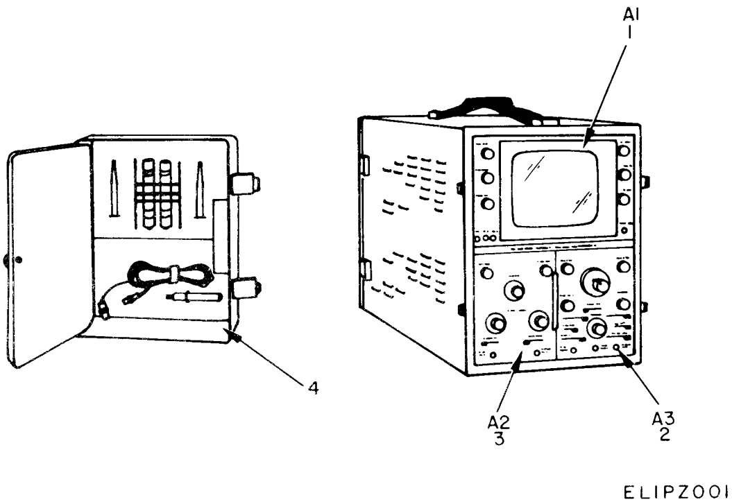
Figure 1. Oscilloscope AN/USM-281A.
